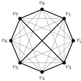
Fig. 6. The graph C_8^{++} bounding \mathcal{SP}_5 (black edges). The gray edges are the weight 2-edges in its corresponding partial distance graph having the all 2-good triple property.
