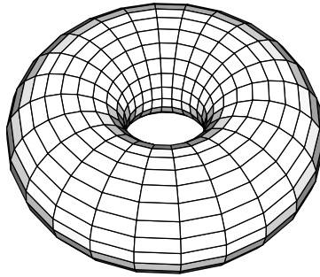
Fig. 2. A representation of the 24 \times 24 toroidal grid.
