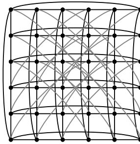
Fig. 3. The augmented toroidal grid AT(6,6) . Gray edges belong to AT(6,6) but not to T(6,6) .
