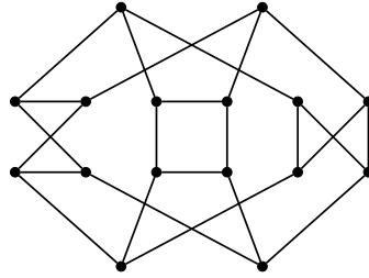
Fig. 7. A 16-vertex bound for \mathcal{SP}_7 .
