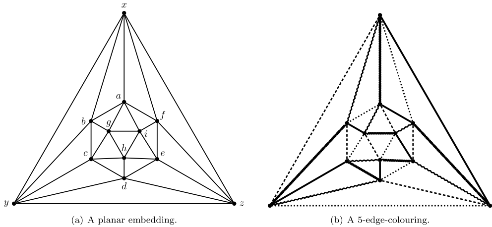
Fig. 10. The Icosahedral graph and a 5-edge-colouring of it.
