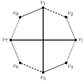
Fig. 9. The 5-edge-colouring of C_8^{++} induced by the canonical edge-colouring of PC(4) .
