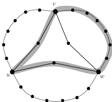
Fig. 1. The graph T_9(2, 2, 2) ; an 11-cycle goes through u, v, w .
