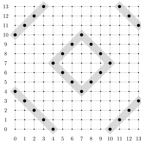
Fig. 4. Illustration of the set N_{AT}^4((0,0)) for k = 7 .
