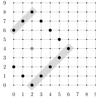
Fig. 5. Illustration of the subset of N_{AT}^4((2, 4)) \cap S^* (in gray) described in Claim 30.A for k = 9 . The large dots are the vertices of N_{AT}^4((2, 4)) \cap S^* .
