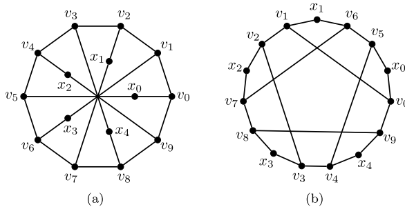
Fig. 8. Two drawings of the graph X_{15} , an optimal 15-vertex bound for \mathcal{SP}_7 .
