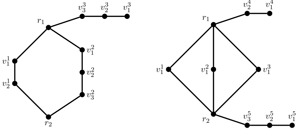
Figure 2. The partial balloons B(2, 3, \bar{3}) and B(1, 1, 1, \bar{2}, 3) .
