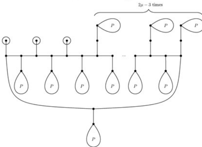
(a) Clause gadget G_{Q_i}(\lambda)
