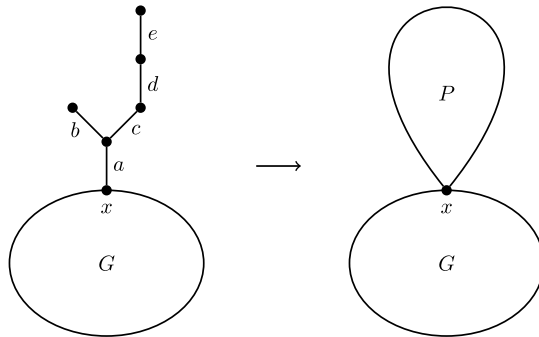
FIGURE 9. The generic P -gadget.
