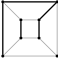
FIGURE 4. An optimal edge-identifying code of \mathcal{H}_3 .
