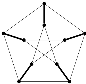
FIGURE 2. An edge-identifying code of the Petersen graph.
