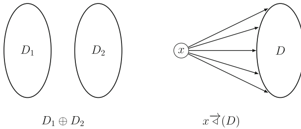
Fig. 1 Illustrations of the two operations
