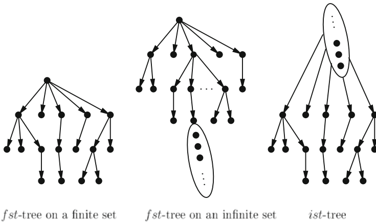
Fig. 2 Underlying trees of source transitive trees
