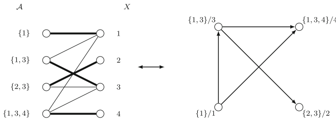
Fig. 3 Digraph of a bipartite graph
