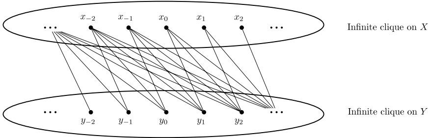
Fig. 2. The graph A_\infty which needs all its vertices for any identifying code.
