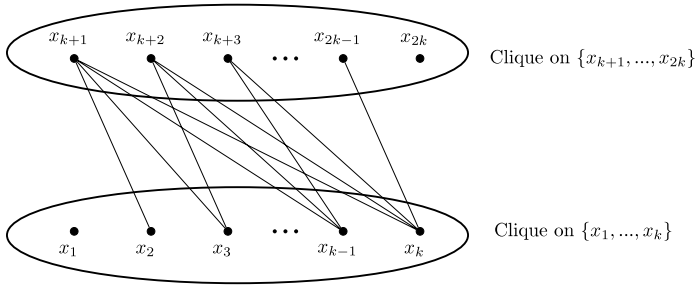
Fig. 1. The graph A_k which needs |V(A_k)| - 1 vertices for any identifying code.
