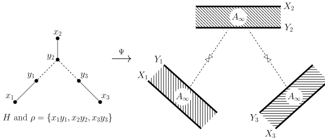
Fig. 3. Construction of \Psi(H, \rho) from (H, \rho) .
